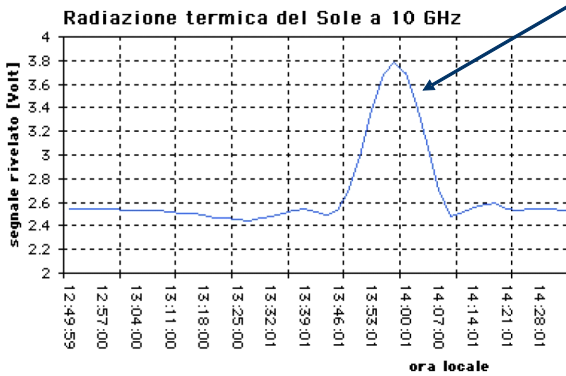
Thermal component of the solar radiation
